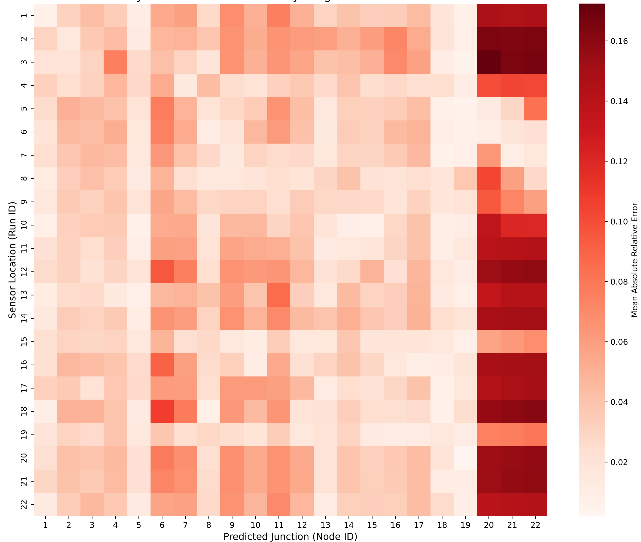
Anytown: Predictive Error by Single Sensor Placement
